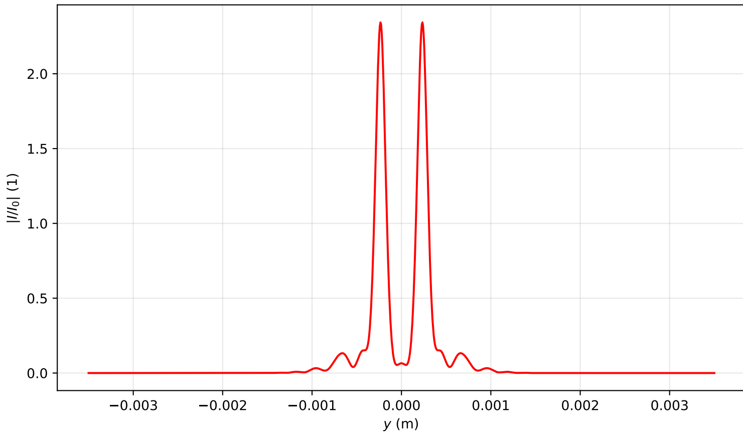
Intensity profile I(x=0, y, z=0.716)/I_0 , P_{in}=5.5P_{cr} , artificial time
